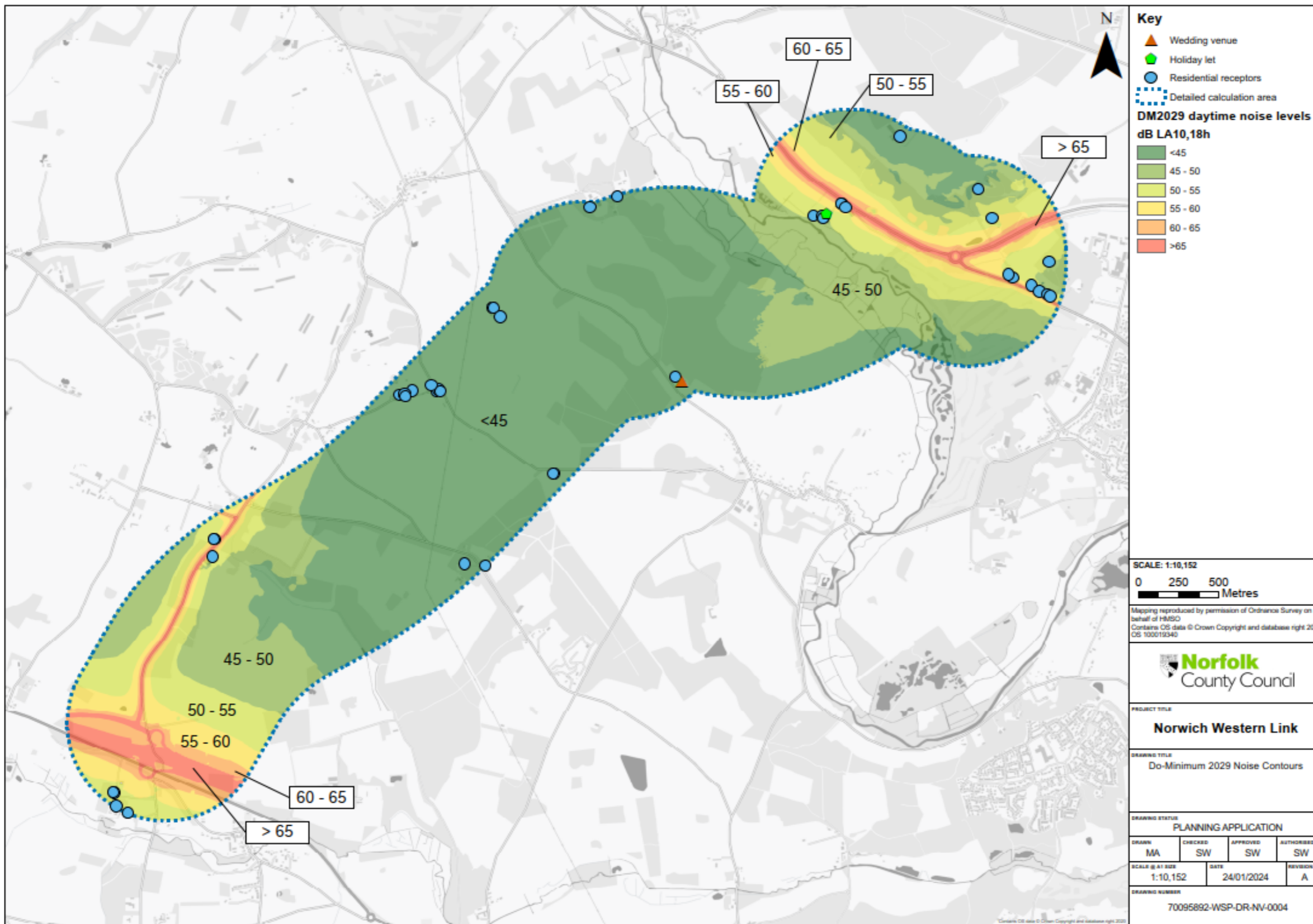
Figure 7.4 Do-Minimum 2029 Noise Contours
