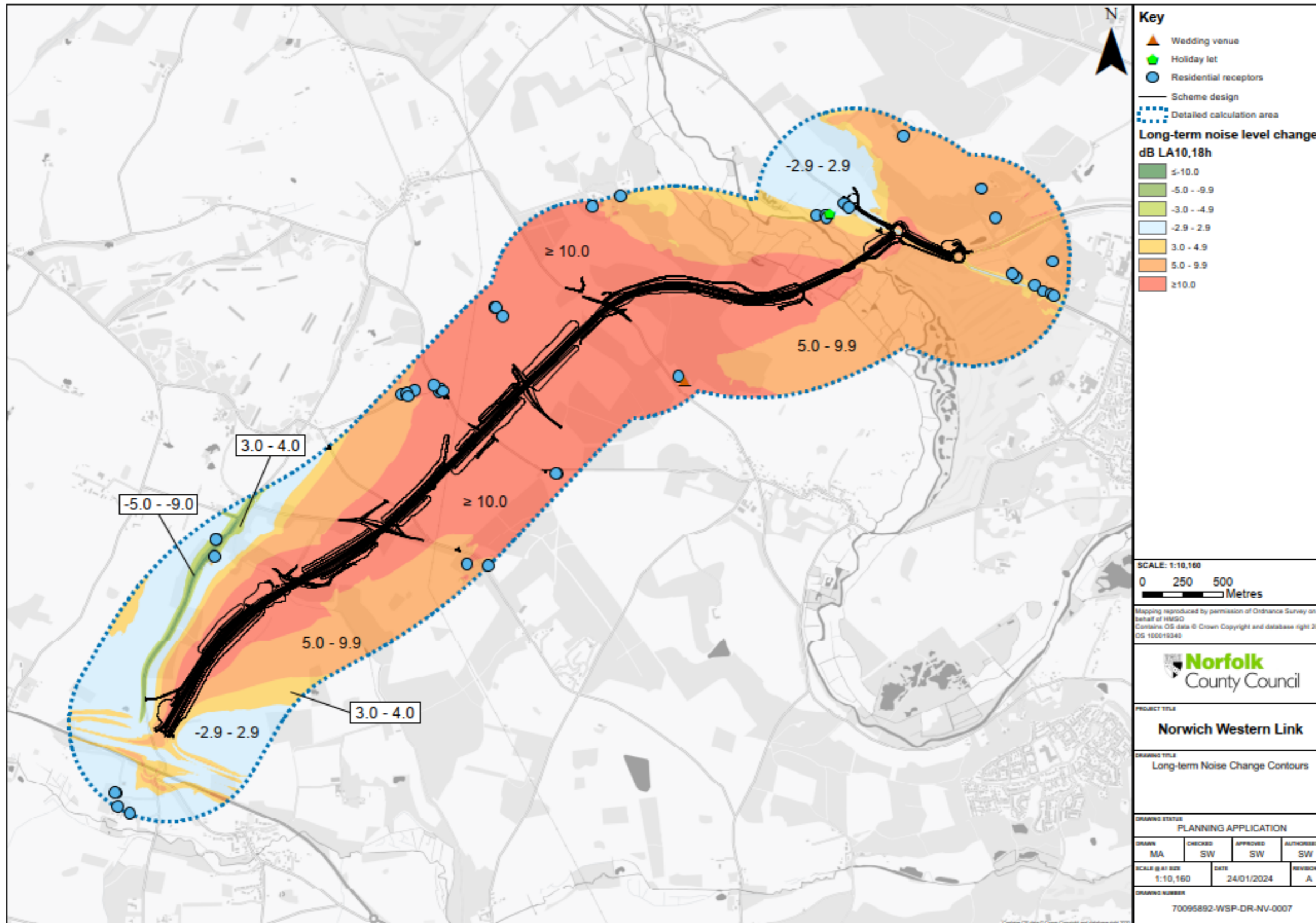
Figure 7.7 Long-Term Noise Change Contours
