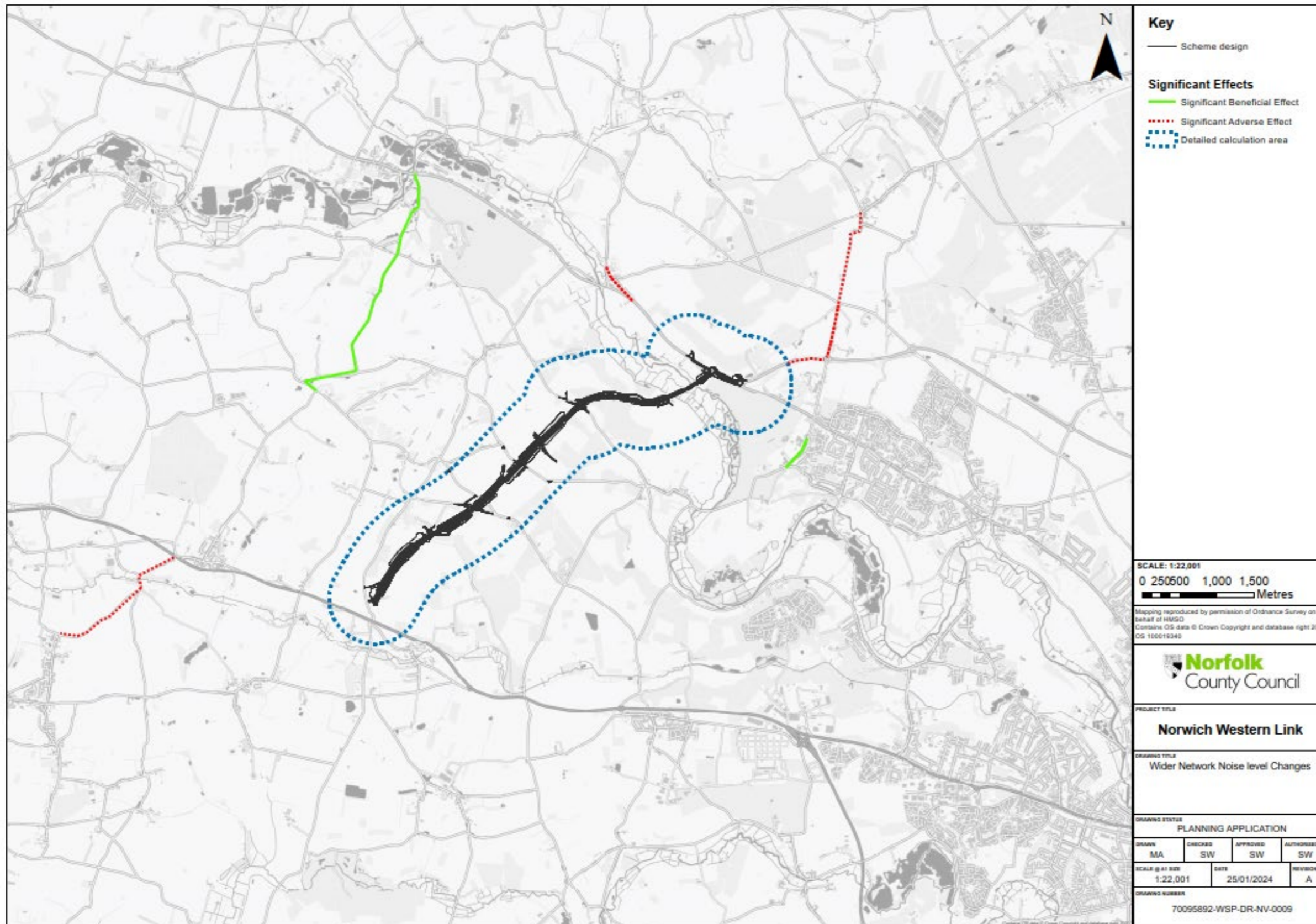
Figure 7.9 Wider Network Noise Level Changes
